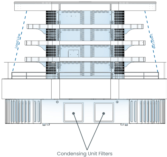
Case Front (Intake)
