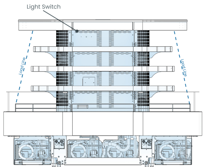
Case Rear-With Lower Panels Removed
