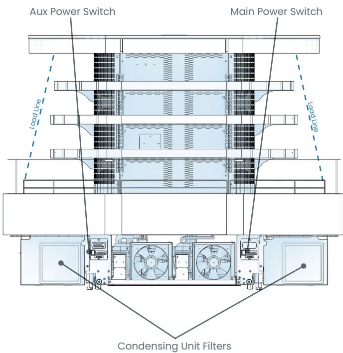
Case Front-With Lower Panels Removed
