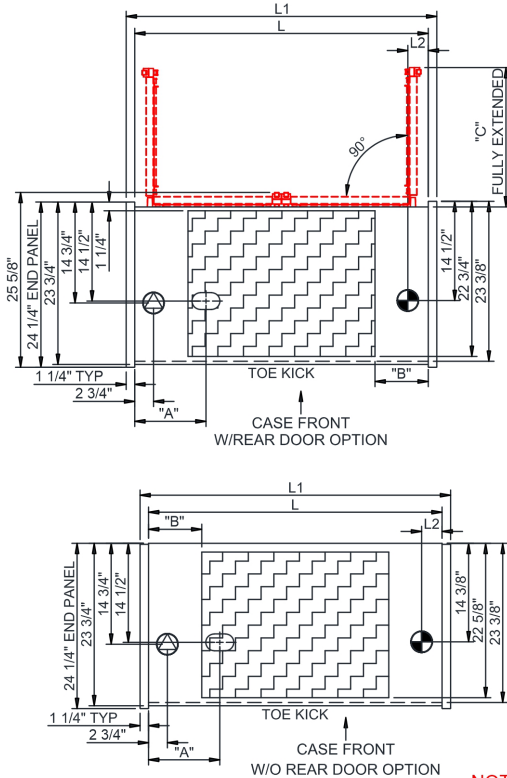
PLAN VIEW
